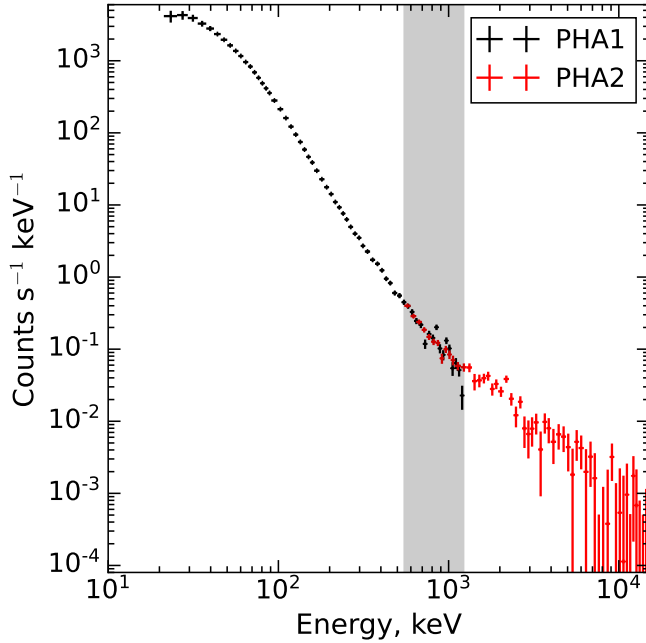
Figure 6. Example of background-subtracted multichannel energy spectrum for the X9.3 class solar flare 2017-09-06 in the first energy range (PHA1, black) and the second energy range (PHA2, red). The gray shaded area marks the PHA1/PHA2 overlapping range.
