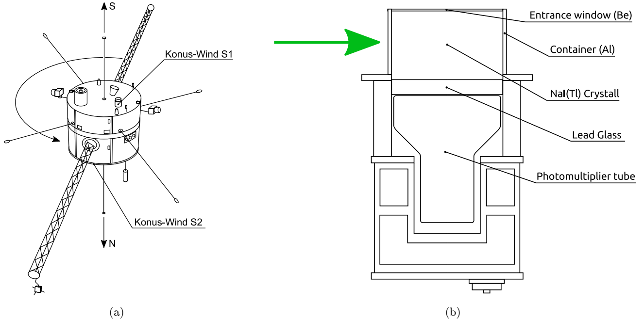
Figure 1. Konus- Wind : (a) the location of Konus detectors S1 and S2 on the spacecraft, “N” and “S” are the directions to the ecliptic poles and the circular arrow indicates the spin direction of the spacecraft; (b) a scheme of the Konus detector. The green arrow indicates the direction of solar emission.
